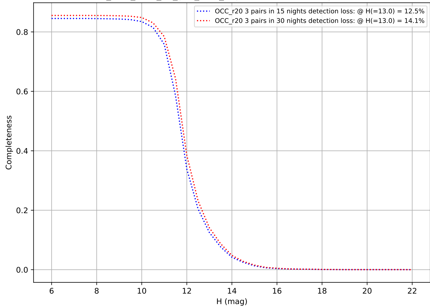
too_elab_r128_d3_griz_v3.4_10yrs: DifferentialCompleteness
