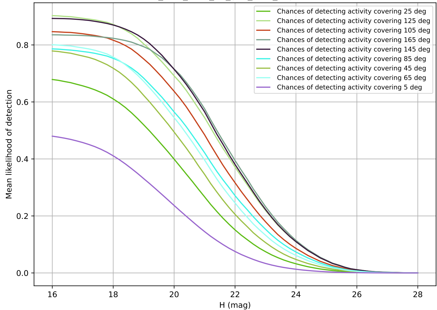
too_elab_r128_d3_griz_v3.4_10yrs NEO
