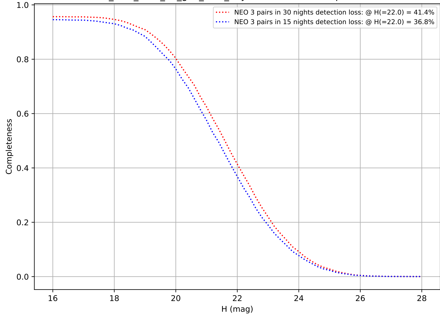
too_elab_r128_d3_griz_v3.4_10yrs: DifferentialCompleteness
