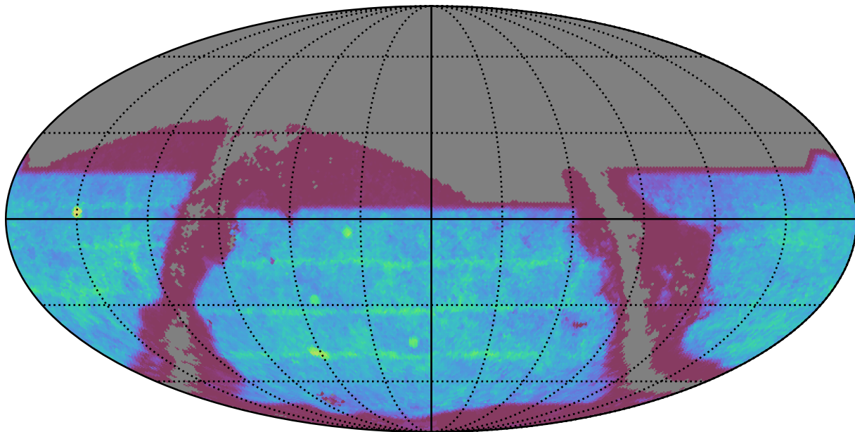
too_elab_r128_d3_griz_v3.4_10yrs : SNSLMetric
