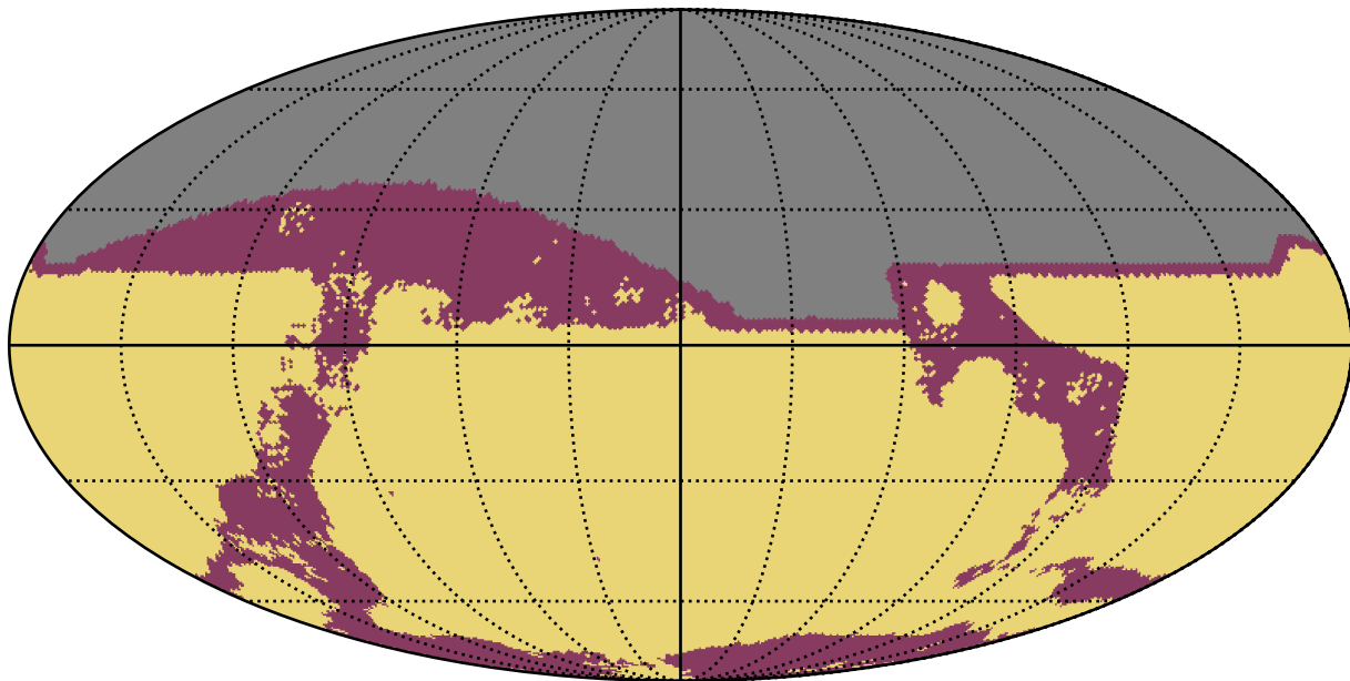
too_elab_r128_d3_griz_v3.4_10yrs : RapidRevisits
