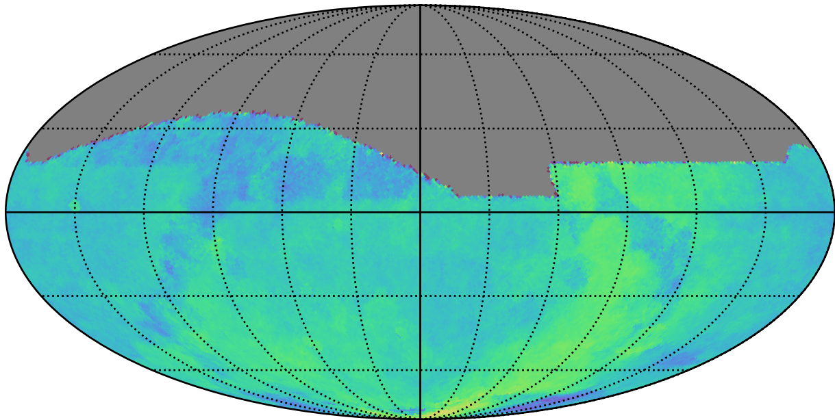
too_elab_r128_d3_griz_v3.4_10yrs : Parallax Coverage @ 22.4
