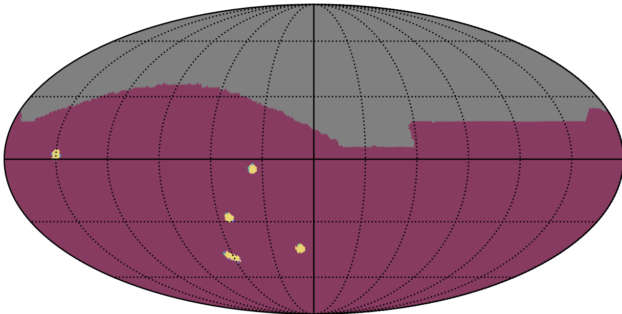
too_elab_r128_d3_griz_v3.4_10yrs : NumberOfQuickRevisits
