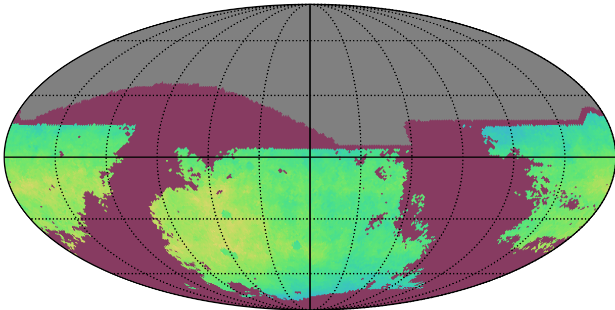
too_elab_r128_d3_griz_v3.4_10yrs i: NgalScale
