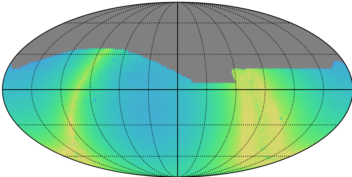
too_elab_r128_d3_griz_v3.4_10yrs i: N stars to Precision 0.20
