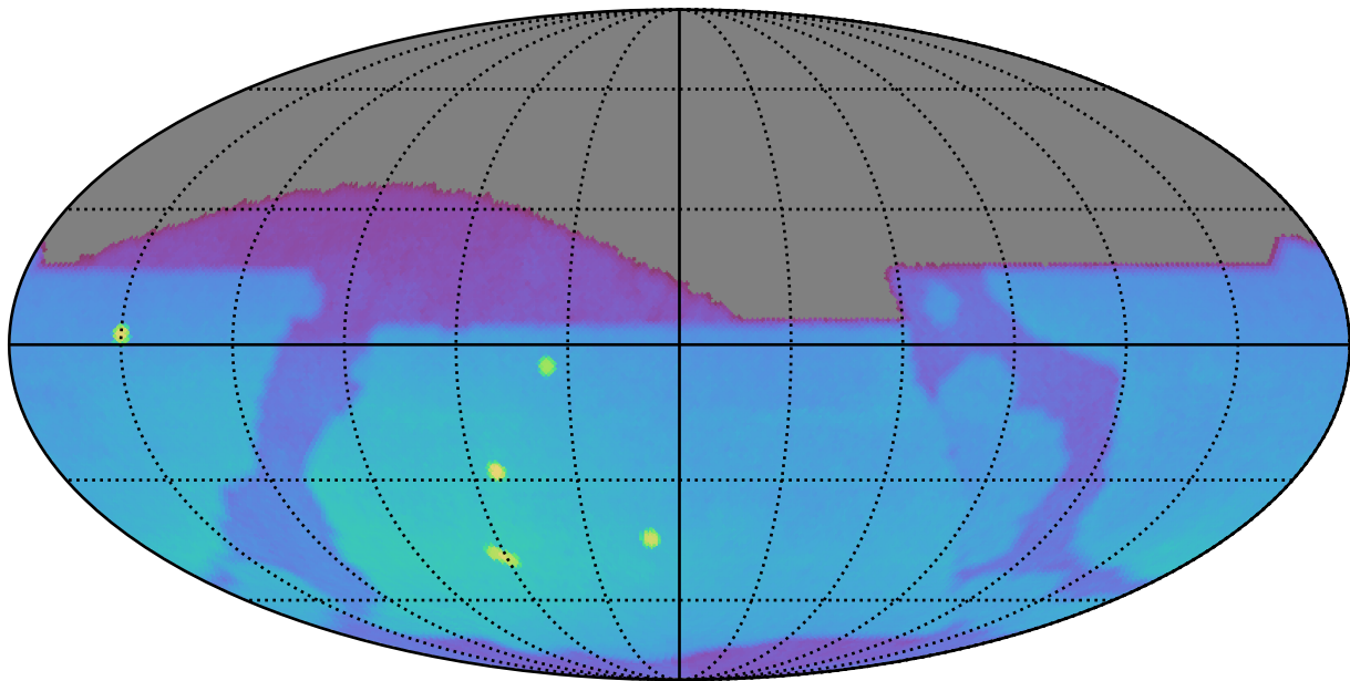
too_elab_r128_d3_griz_v3.4_10yrs : Brown Dwarf, L4
