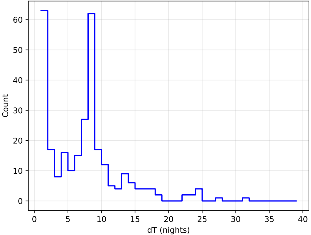
too_elab_r128_d3_griz_v3.4_10yrs all bands: DD:XMM_LSS Delta Nights Histogram
