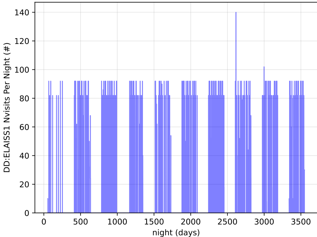
too_elab_r128_d3_griz_v3.4_10yrs all bands: DD:ELAISS1 Nvisits Per Night
