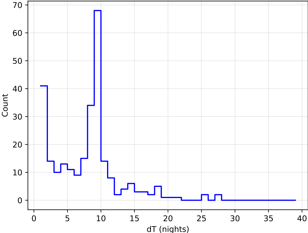
too_elab_r128_d3_griz_v3.4_10yrs all bands: DD:ELAISS1 Delta Nights Histogram
