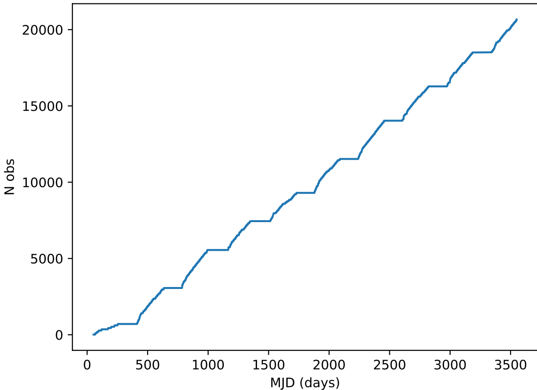
too_elab_r128_d3_griz_v3.4_10yrs all bands: DD:ELAISS1 Cumulative NVisits
