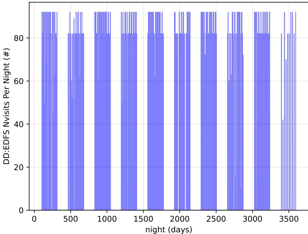
too_elab_r128_d3_griz_v3.4_10yrs all bands: DD:EDFS Nvisits Per Night
