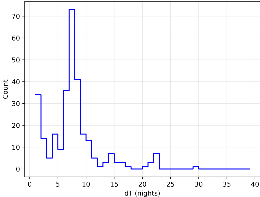
too_elab_r128_d3_griz_v3.4_10yrs all bands: DD:EDFS Delta Nights Histogram
