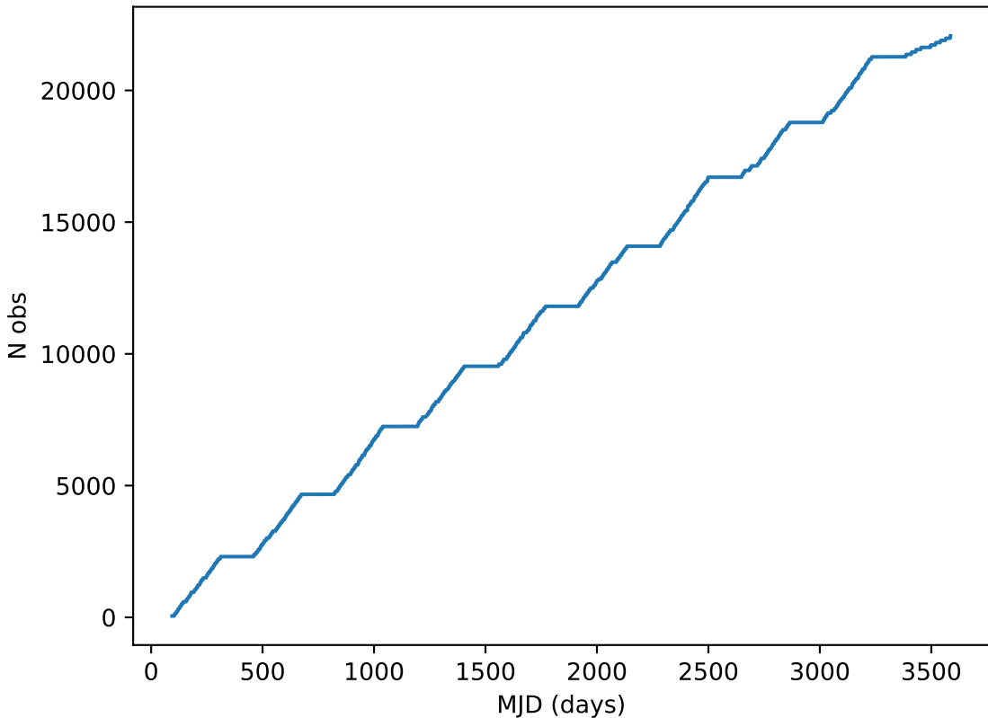
too_elab_r128_d3_griz_v3.4_10yrs all bands: DD:ECDFS Cumulative NVisits
