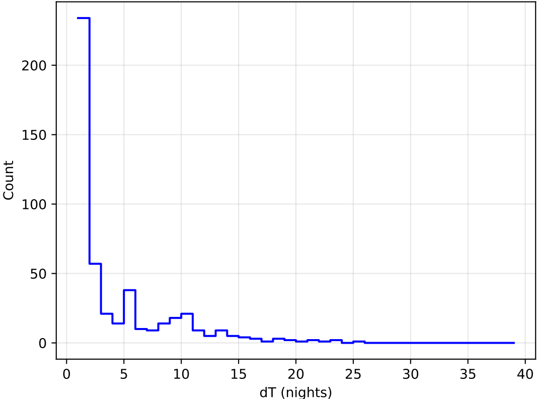
too_elab_r128_d3_griz_v3.4_10yrs all bands: DD: COSMOS Delta Nights Histogram
