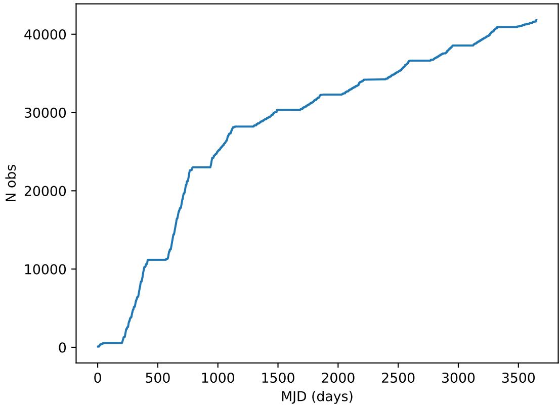
too_elab_r128_d3_griz_v3.4_10yrs all bands: DD: COSMOS Cumulative NVisits
