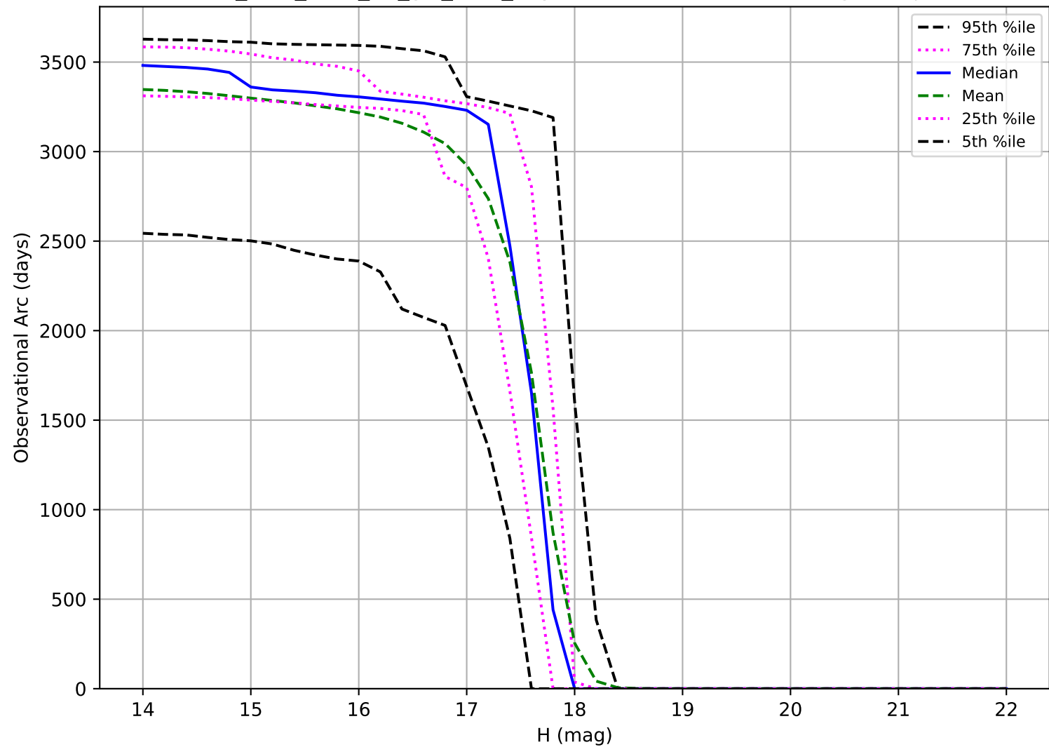
too_elab_r128_d3_giz_v3.4_10yrs: Observational Arc Length Trojan
