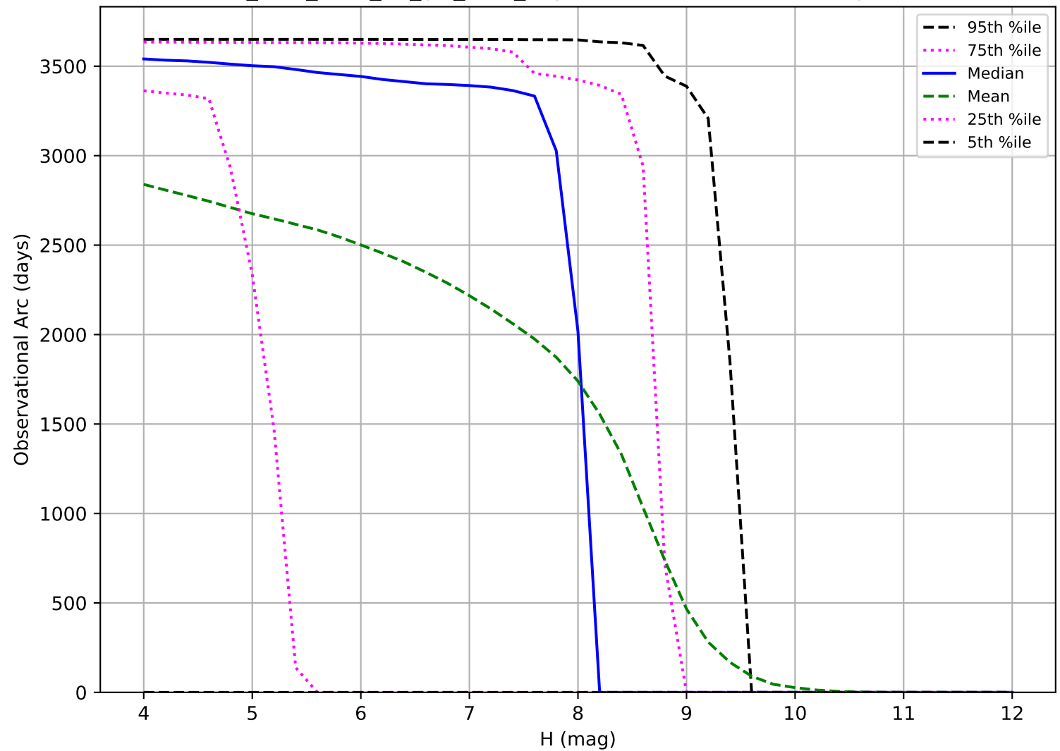
too_elab_r128_d3_giz_v3.4_10yrs: Observational Arc Length TNO
