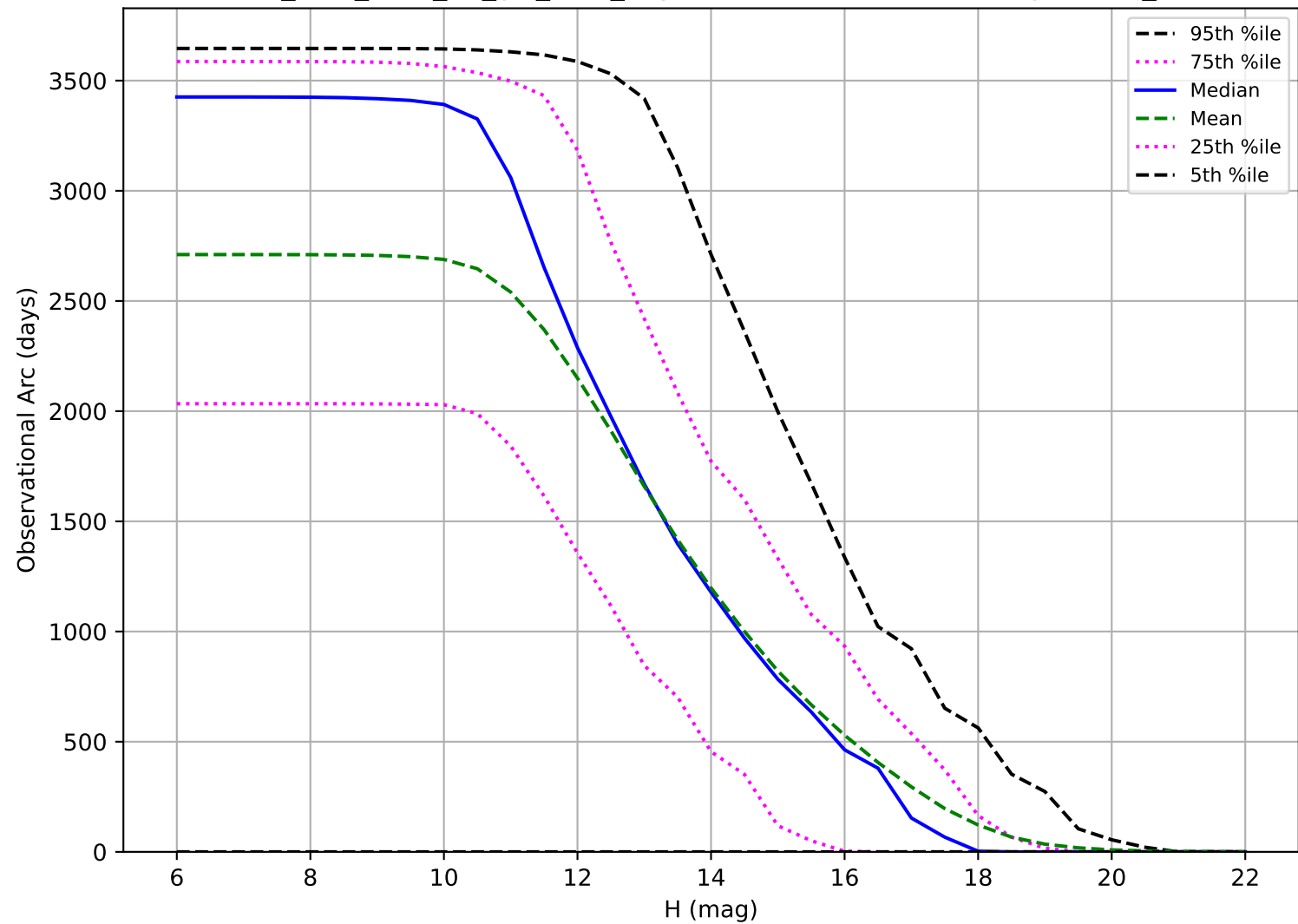
too_elab_r128_d3_giz_v3.4_10yrs: Observational Arc Length OCC_r5
