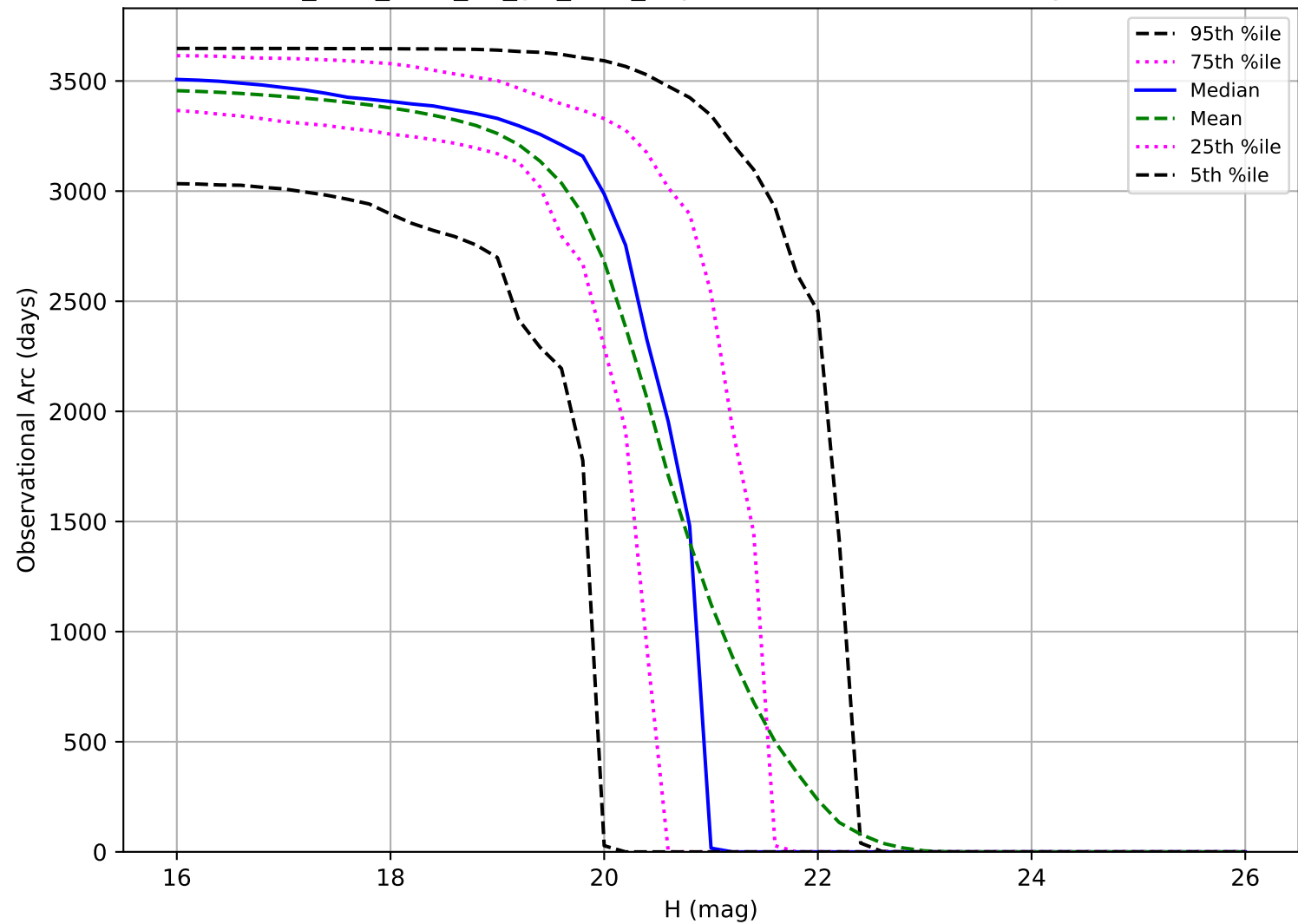
too_elab_r128_d3_giz_v3.4_10yrs: Observational Arc Length MBA
