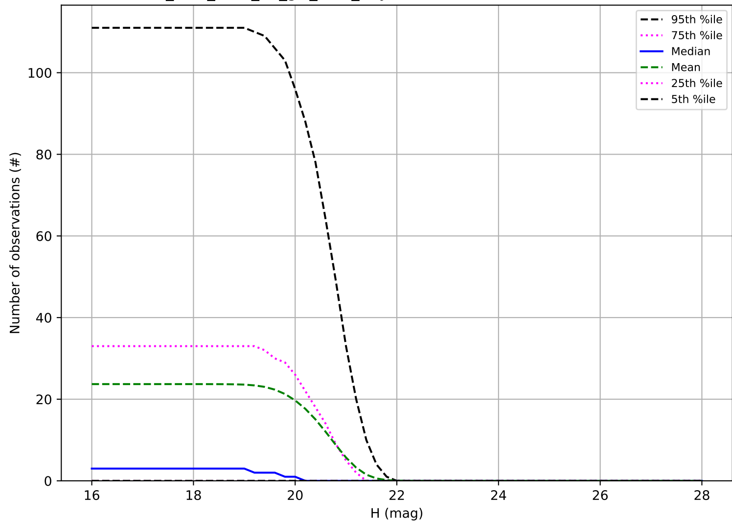
too_elab_r128_d3_giz_v3.4_10yrs: Number of observations Vatira
