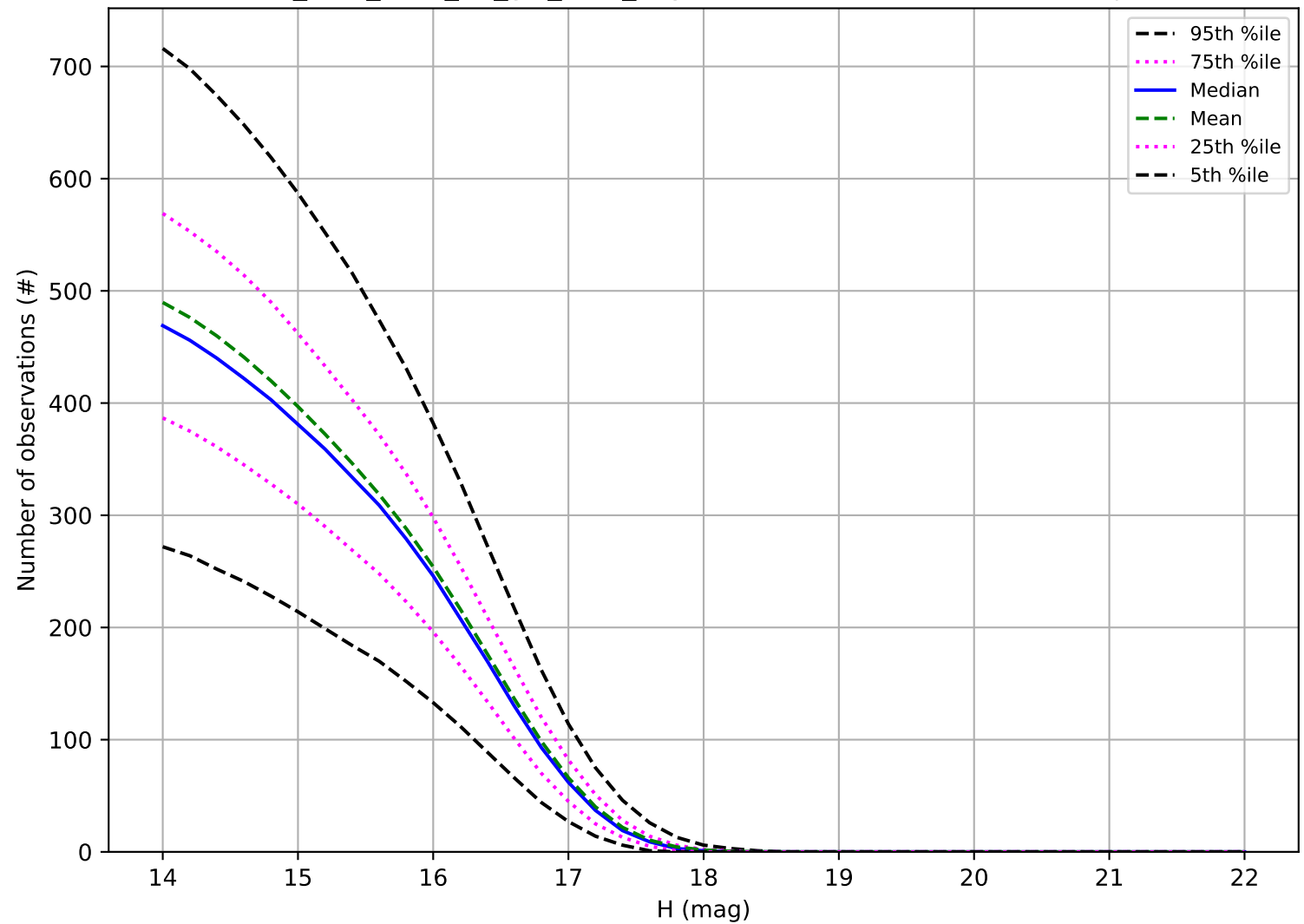
too_elab_r128_d3_giz_v3.4_10yrs: Number of observations Trojan
