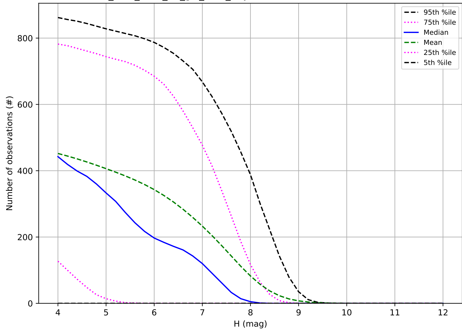
too_elab_r128_d3_giz_v3.4_10yrs: Number of observations TNO
