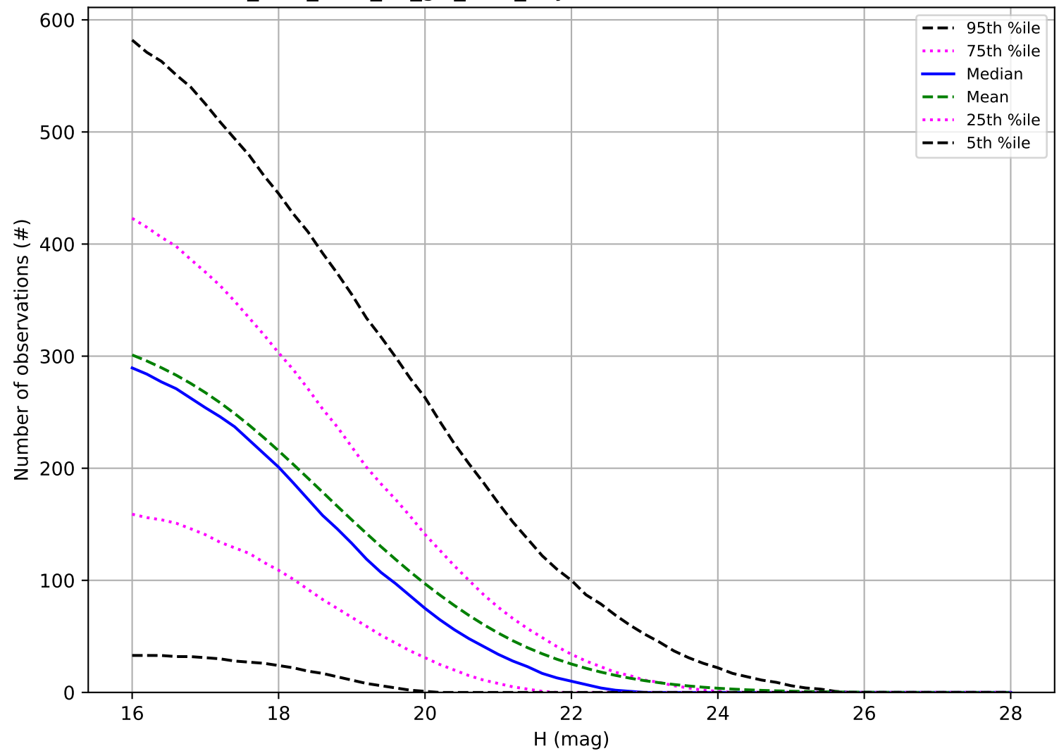
too_elab_r128_d3_giz_v3.4_10yrs: Number of observations NEO
