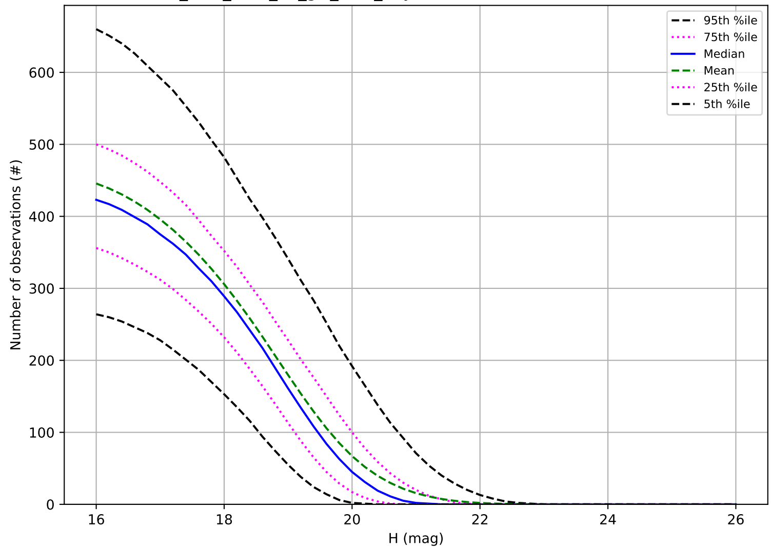
too_elab_r128_d3_giz_v3.4_10yrs: Number of observations MBA
