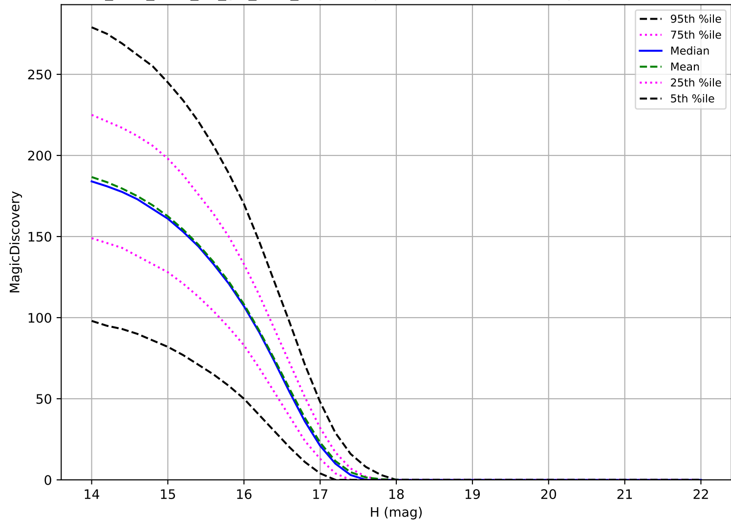
too_elab_r128_d3_giz_v3.4_10yrs: Trojan 6 detections in 60 nights detection loss
