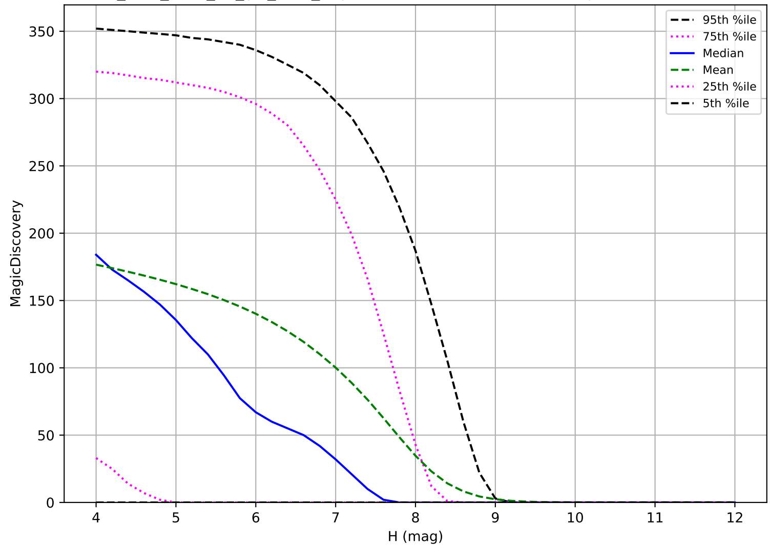
too_elab_r128_d3_giz_v3.4_10yrs: TNO 6 detections in 60 nights detection loss
