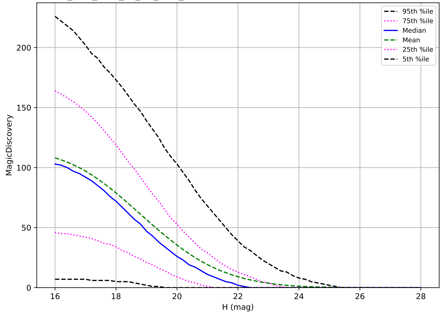
too_elab_r128_d3_giz_v3.4_10yrs: PHA 6 detections in 60 nights detection loss
