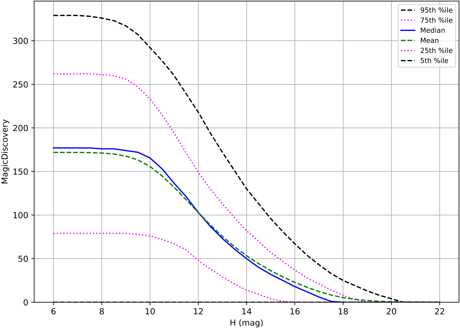
too_elab_r128_d3_giz_v3.4_10yrs: OCC_r5 6 detections in 60 nights detection loss
