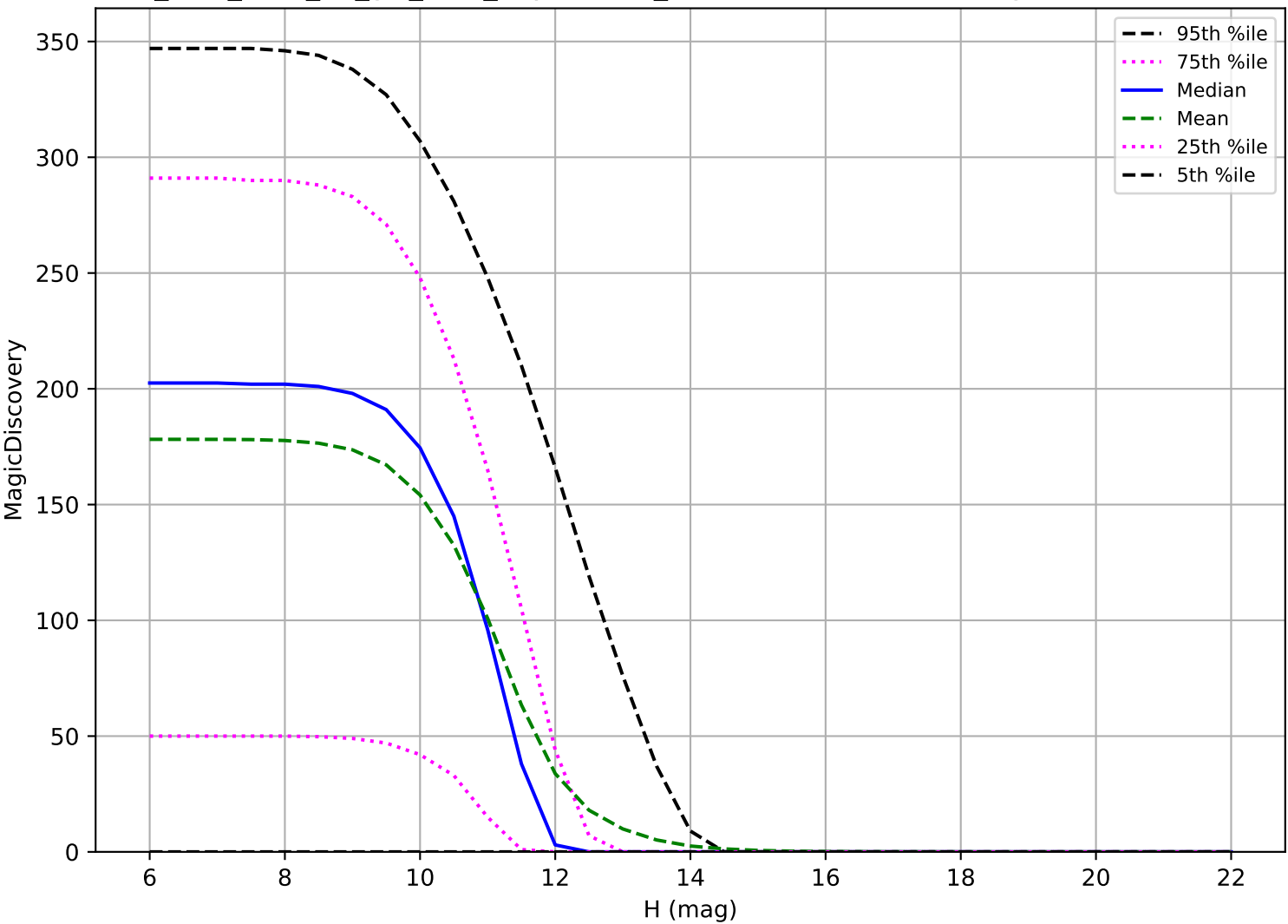
too_elab_r128_d3_giz_v3.4_10yrs: OCC_r20 6 detections in 60 nights detection loss
