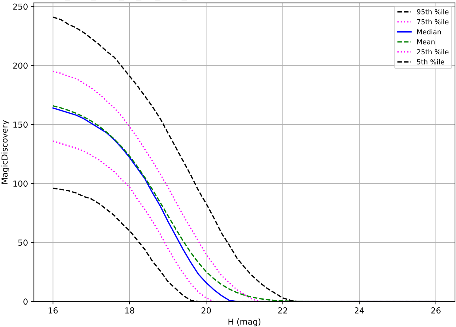
too_elab_r128_d3_giz_v3.4_10yrs: MBA 6 detections in 60 nights detection loss
