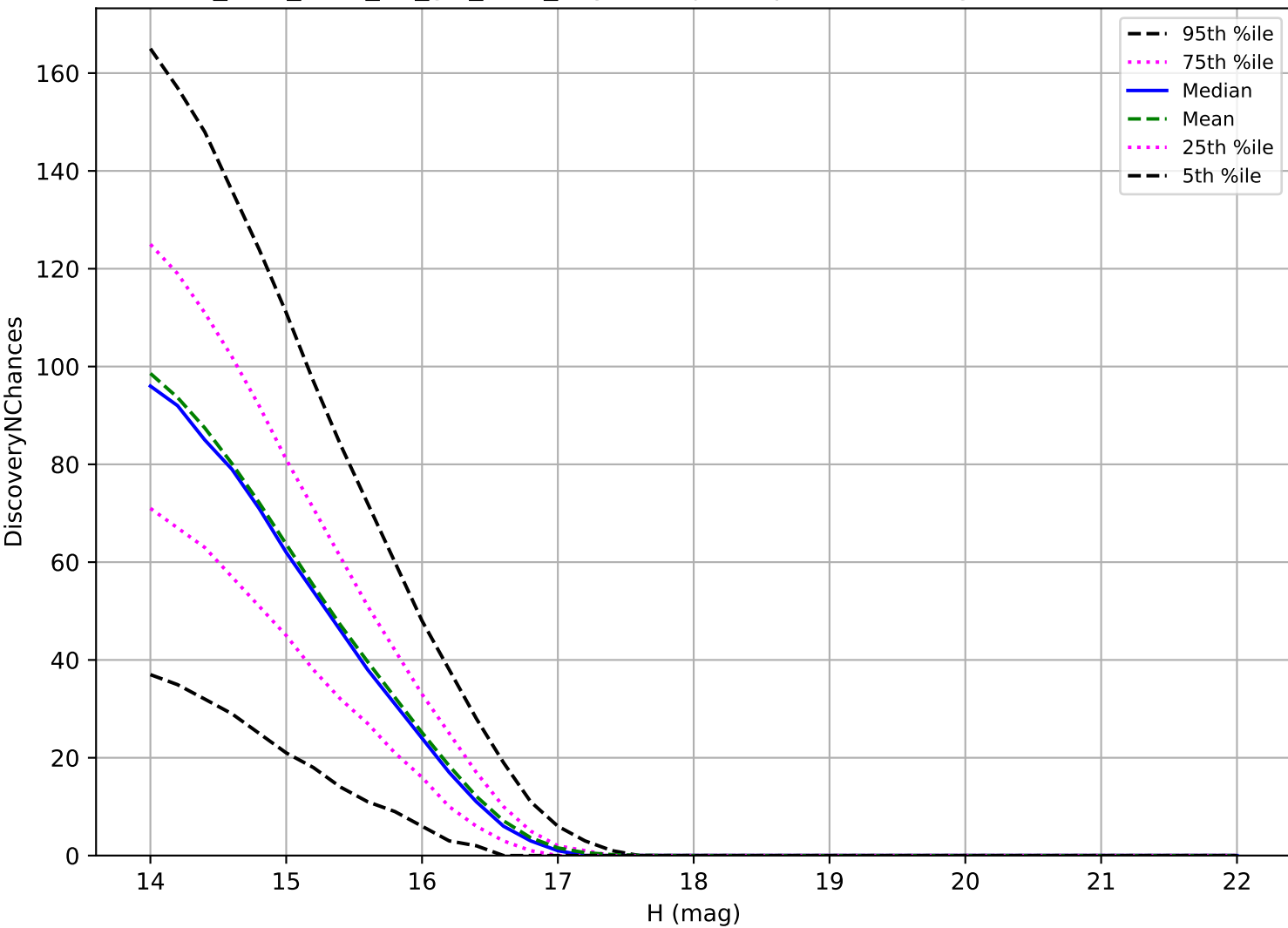
too_elab_r128_d3_giz_v3.4_10yrs: Trojan 3 pairs in 15 nights detection loss
