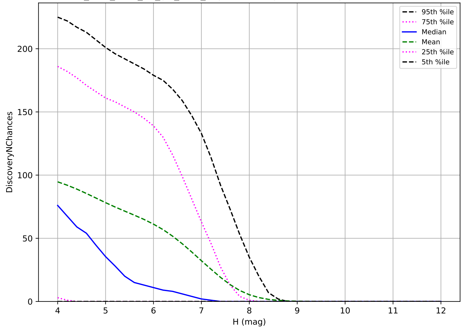
too_elab_r128_d3_giz_v3.4_10yrs: TNO 3 pairs in 15 nights detection loss
