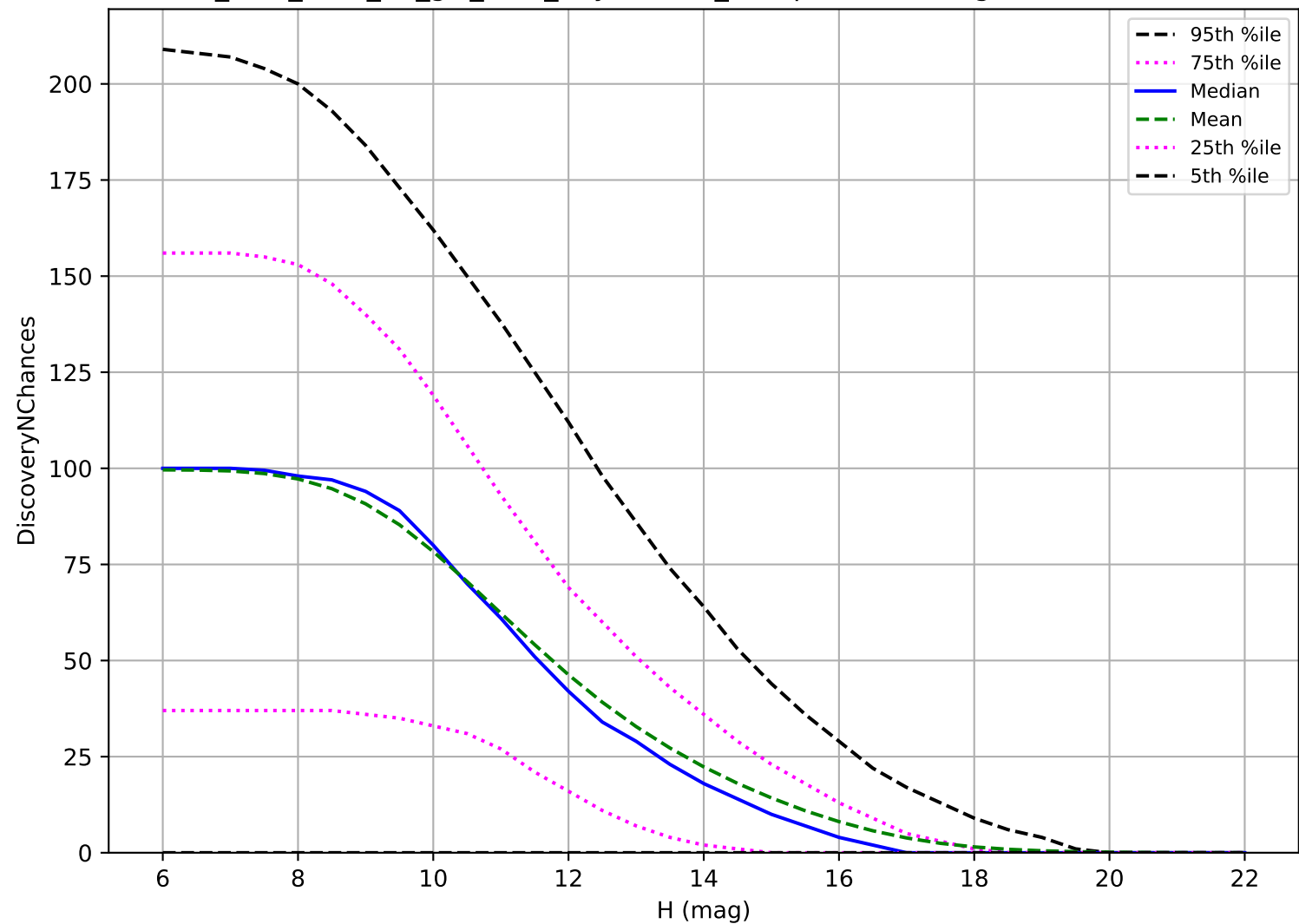
too_elab_r128_d3_giz_v3.4_10yrs: OCC_r5 3 pairs in 15 nights detection loss
