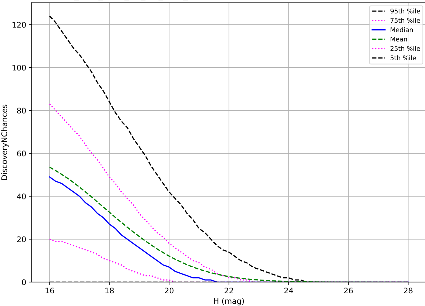
too_elab_r128_d3_giz_v3.4_10yrs: NEO 3 pairs in 15 nights detection loss
