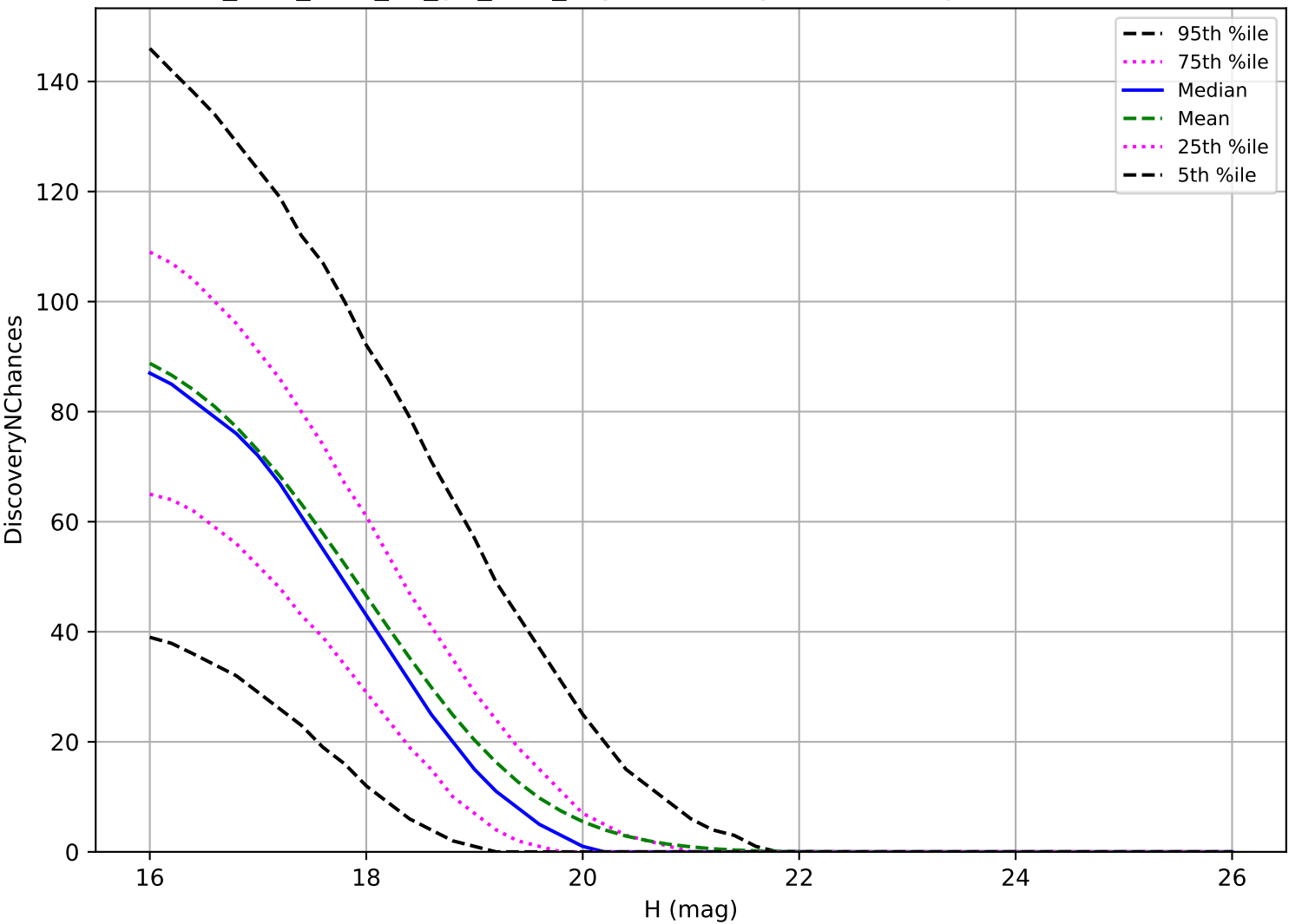
too_elab_r128_d3_giz_v3.4_10yrs: MBA 3 pairs in 15 nights detection loss
