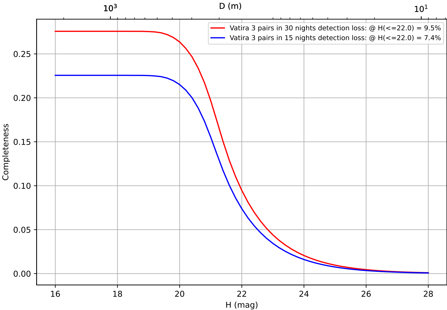
too_elab_r128_d3_giz_v3.4_10yrs: CumulativeCompleteness
