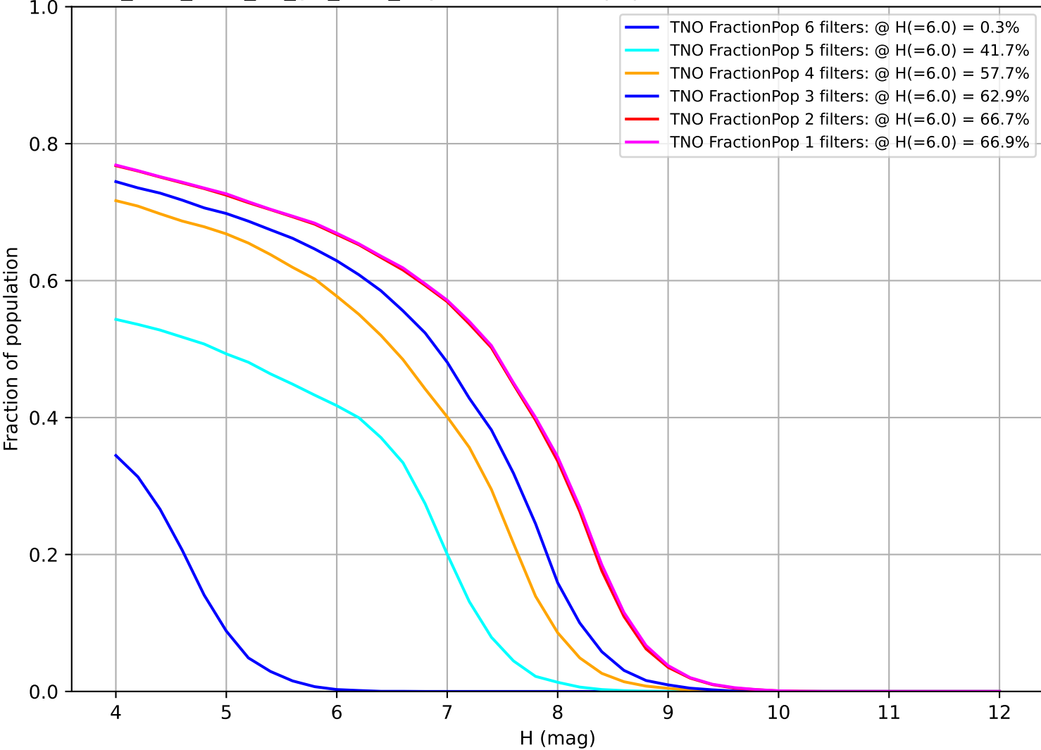
too_elab_r128_d3_giz_v3.4_10yrs: Fraction of population with colors in X filters TNO
