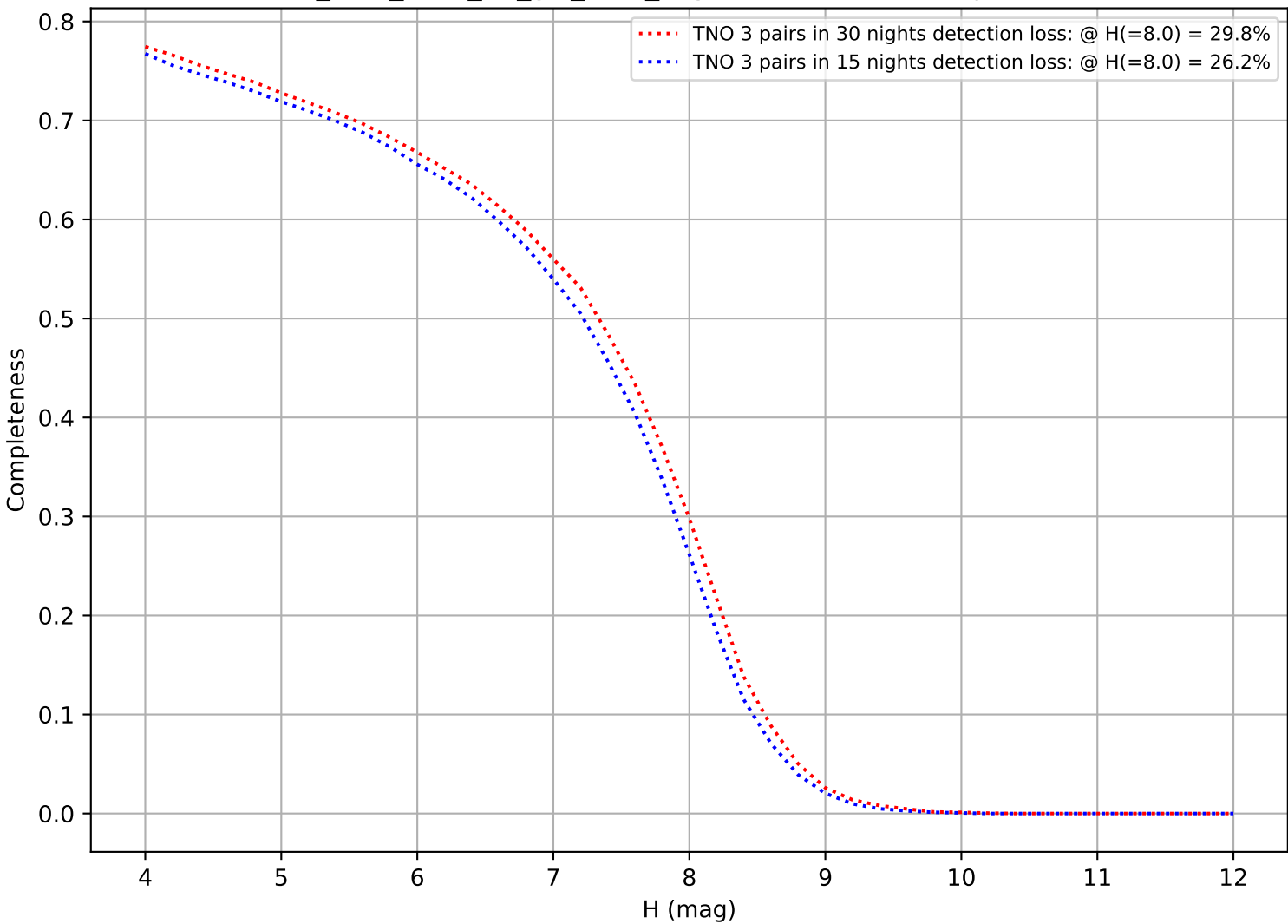
too_elab_r128_d3_giz_v3.4_10yrs: DifferentialCompleteness
