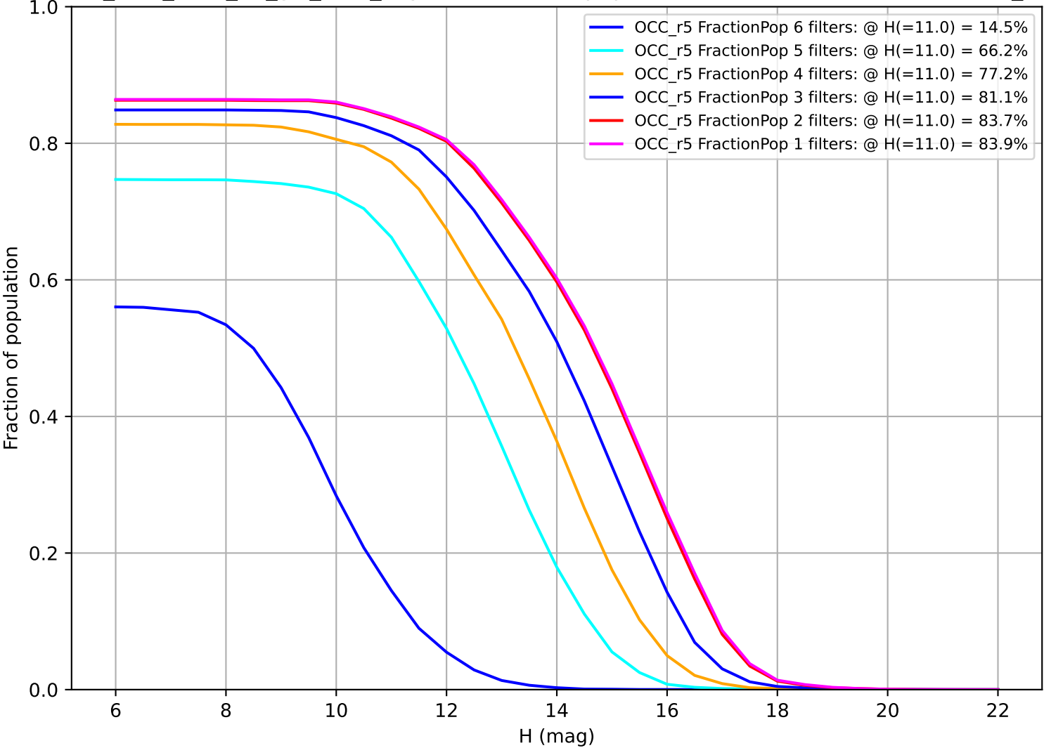
too_elab_r128_d3_giz_v3.4_10yrs: Fraction of population with colors in X filters OCC_r5
