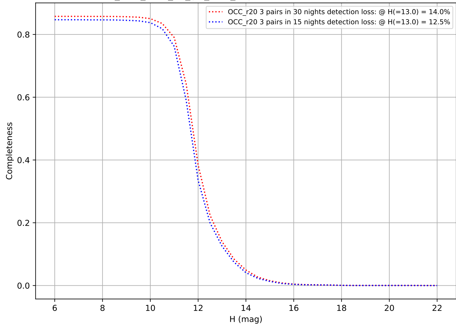
too_elab_r128_d3_giz_v3.4_10yrs: DifferentialCompleteness
