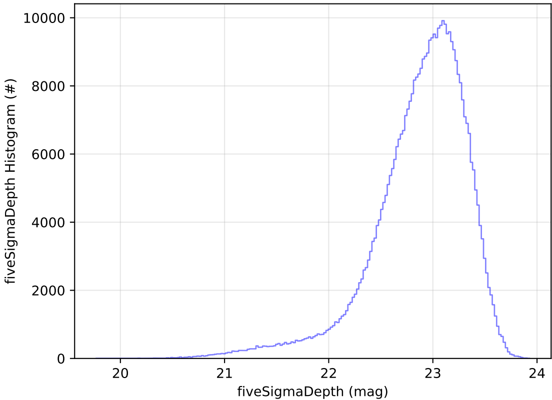
too_elab_r128_d3_giz_v3.4_10yrs z: fiveSigmaDepth Histogram
