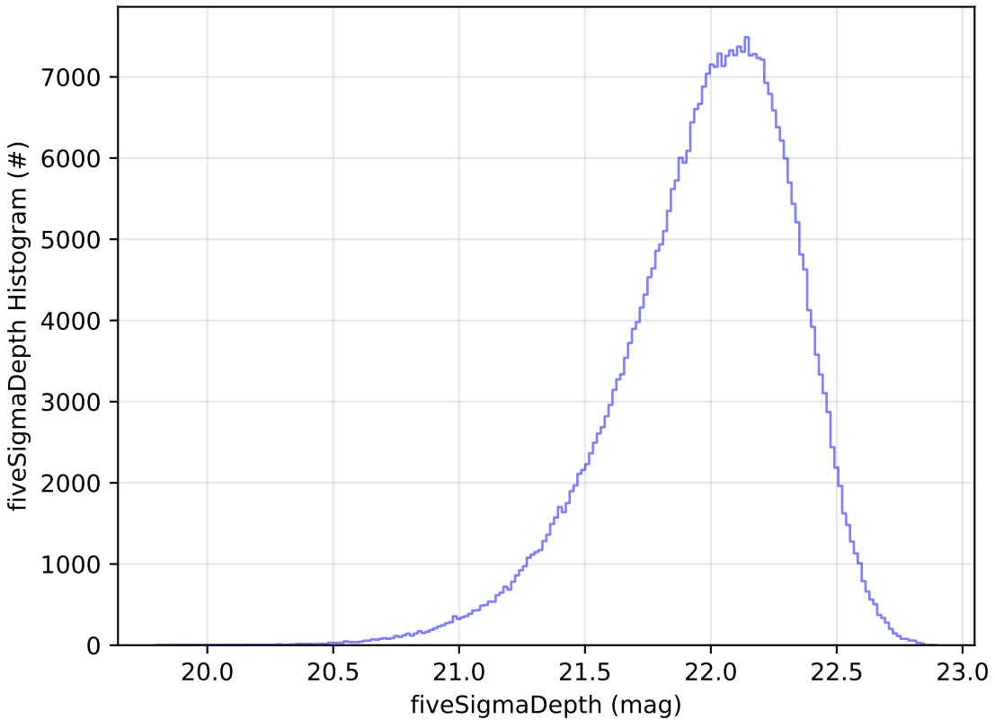
too_elab_r128_d3_giz_v3.4_10yrs y: fiveSigmaDepth Histogram
