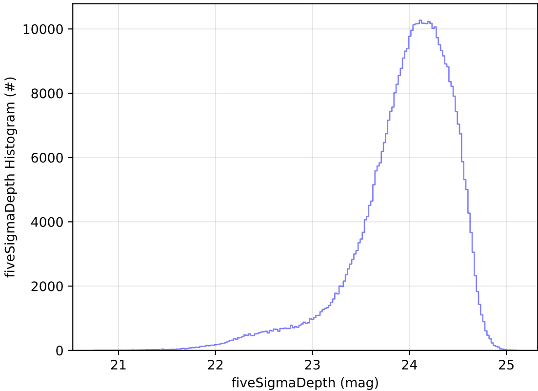
too_elab_r128_d3_giz_v3.4_10yrs r: fiveSigmaDepth Histogram
