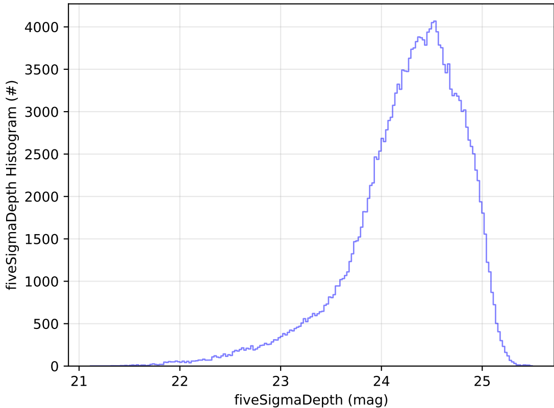
too_elab_r128_d3_giz_v3.4_10yrs g: fiveSigmaDepth Histogram
