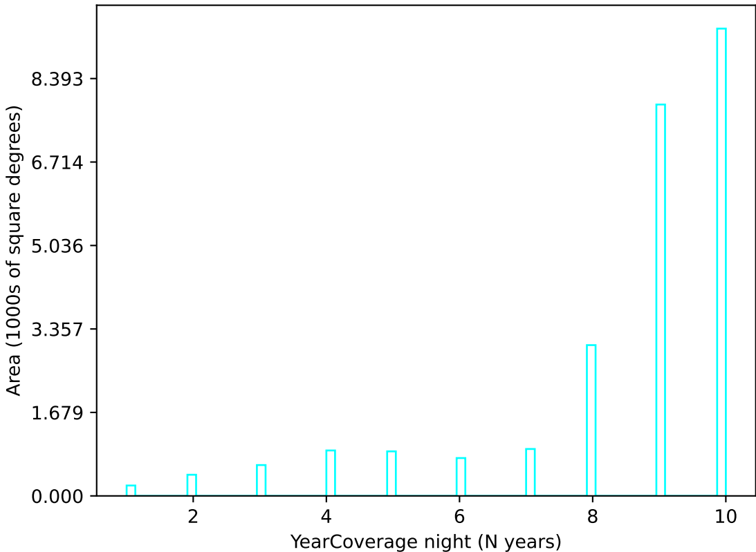
too_elab_r128_d3_giz_v3.4_10yrs u band: YearCoverage night
