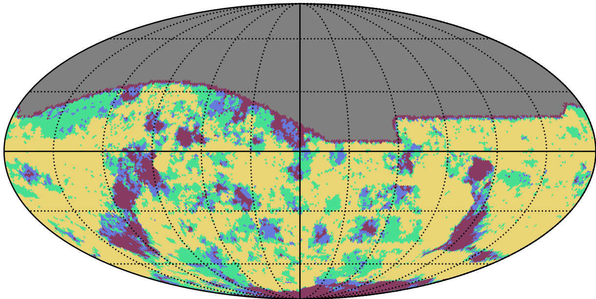
too_elab_r128_d3_giz_v3.4_10yrs g band: YearCoverage night
